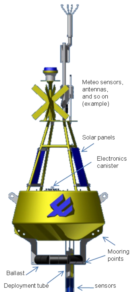
OMC-7012 main components
