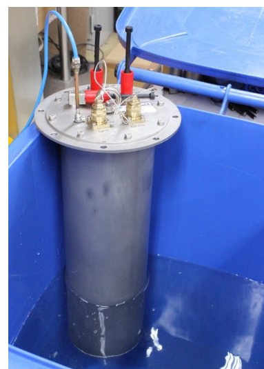
Pressure test of the canister with electronics and battery.
