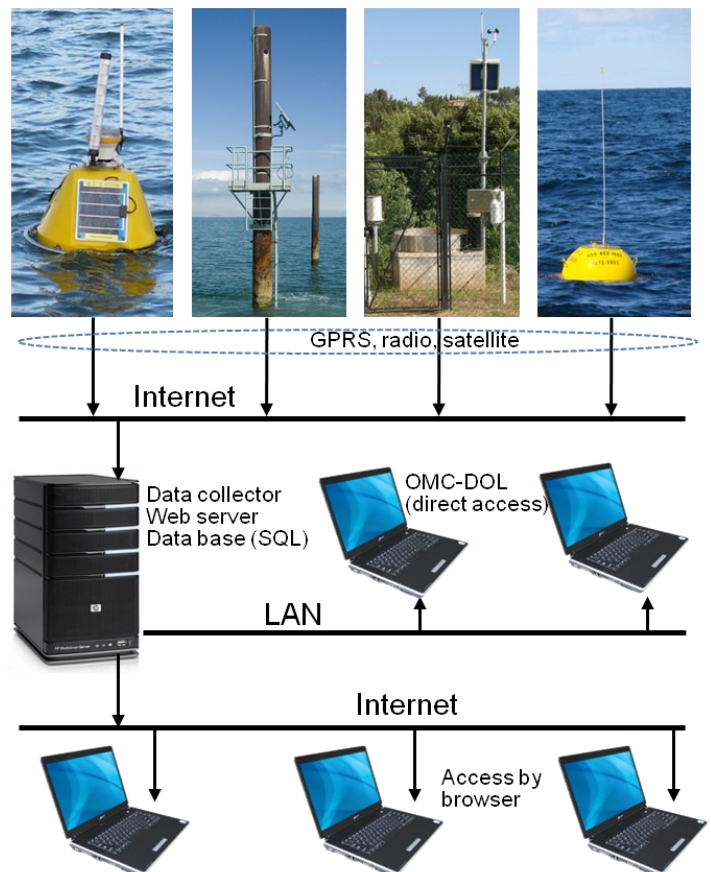
Fig. 4: Typical OMC-DOL application: Multiple stations send data via internet to a server running OMC-DOL. Computers on the LAN can directly access the data. Computers elsewhere in the internet can access the data through a web server.
