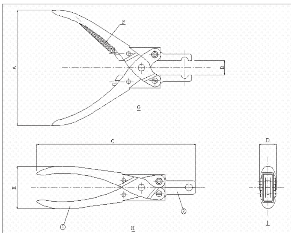
Twine-measuring pliers assembly
